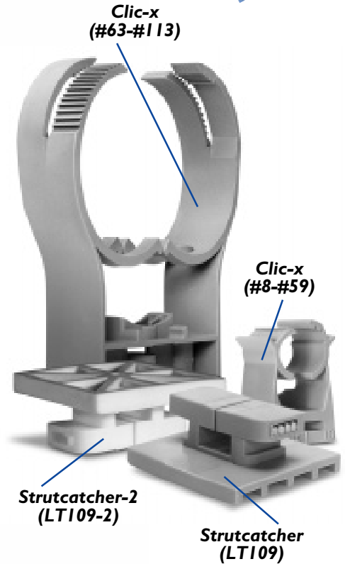
Apply slight pressure to the tubular member and the jaws close and lock.
